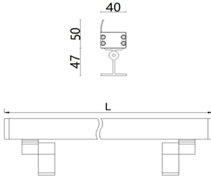
Overall dimensions (mm): body 40 (W) × 47 (H); 50 mm overall height with adjustable bracket.
