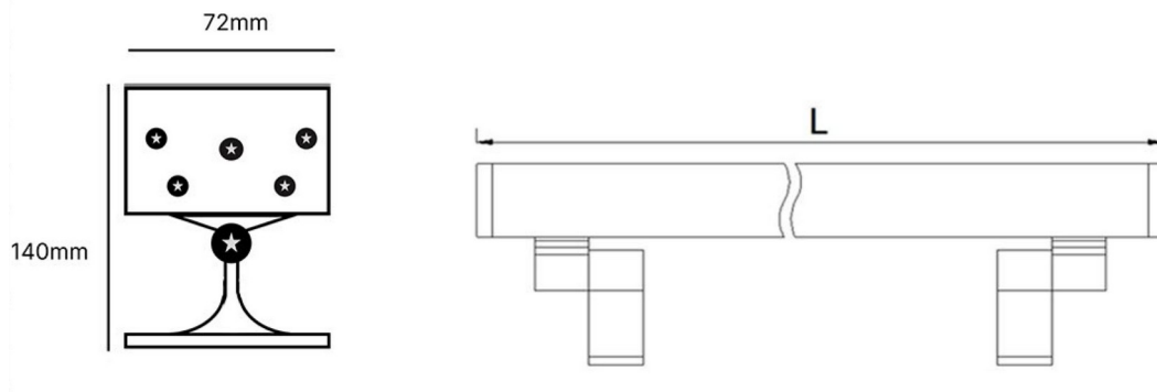
Overall dimensions (mm): body 72 (W), 140 mm overall height with adjustable bracket.
