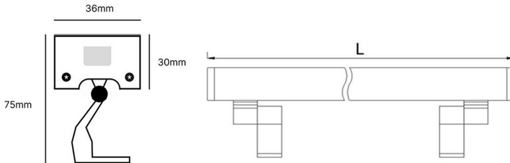
Overall dimensions (mm): body 36 (W) × 30 (H), 75 mm overall height with adjustable bracket.
